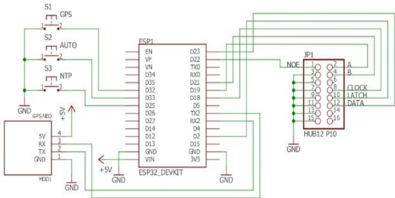
Figure 2. Tool Design Configuration
